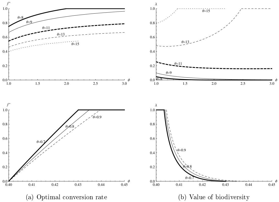
(a) Optimal conversion rate (b) Value of biodiversity Figure 3: Optimal conversion rate and biodiversity value as a function of aversion to fluctuations for \alpha = 0.05 , \rho = 0.03 , \sigma = 0.1 .
