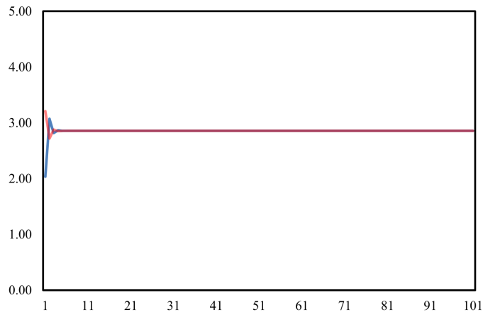
Figure 9: Convergence dynamics of Nash equilibria ( x_u^* , x_v^* ) for \alpha = 0.50 and \phi = 0.80 . The x -axis corresponds to the timeline ( t ). The y -axis denotes the evolution of equilibrium values as a function of time ( x_u^*(t) , x_v^*(t) ).
