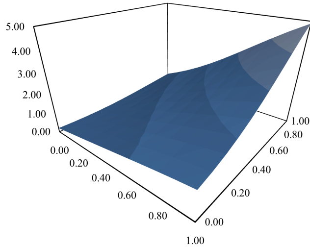
Figure 4: Nash bargaining solution (x_u^*) with heterogeneous expectations. The left-sided x -axis corresponds to the decay parameter of player u ( \alpha_u ). The right-sided y -axis is the decay parameter of player v ( \alpha_v ). The z -axis denotes the equilibrium values.
