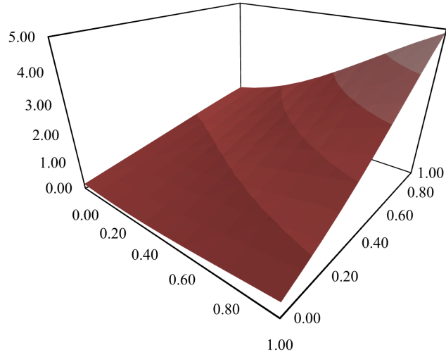
Figure 5: Nash bargaining solution ( x_v^* ) with heterogeneous expectations. The left-sided x -axis corresponds to the decay parameter of player u ( \alpha_u ). The right-sided y -axis is the decay parameter of player v ( \alpha_v ). The z -axis denotes the equilibrium values.
